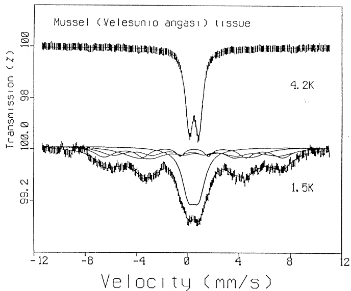
Fig. 9. Mössbauer spectra of tissue granules of freshwater mussel Velusunio angasi at 4.2 and 1.5 K.
